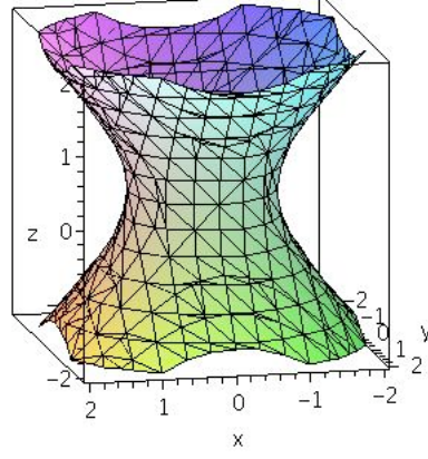
Figure 9.3: A pictorial representation of de Sitter ( X_0^2 - X_1^2 = -l^2 + \vec{X}^2 ) in \mathbb{R}^n ).
