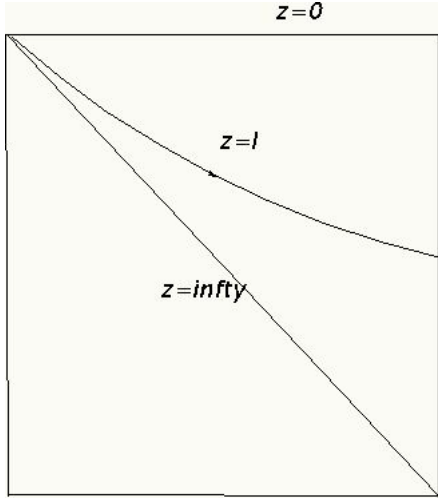
Figure 9.5: Surfaces of constant z in Poincaré coordinates in dS_n .
