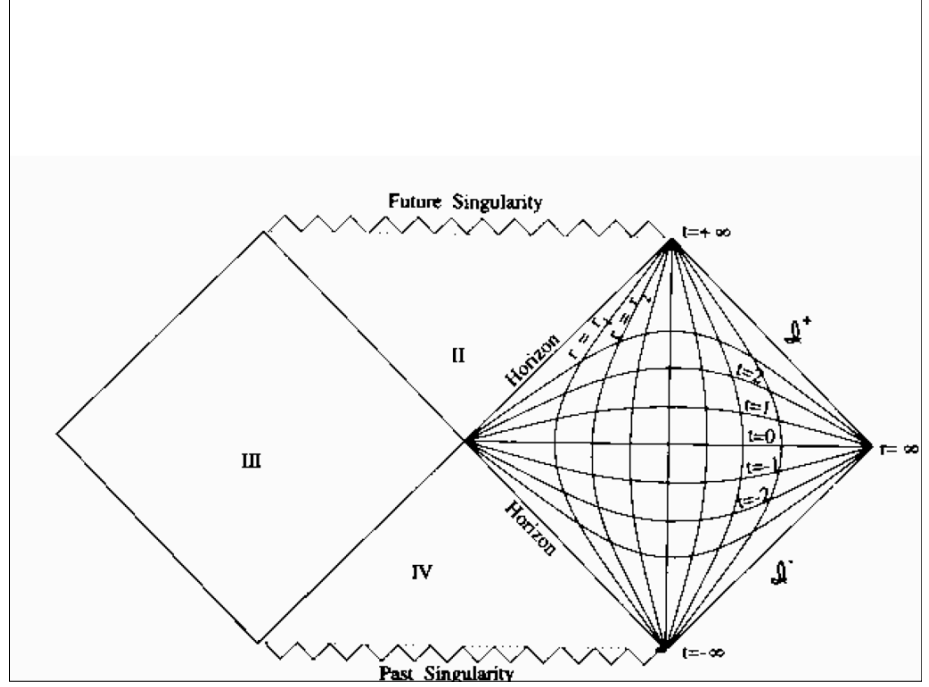
Figure 7.1: Penrose diagram of the Kruskal metric.
