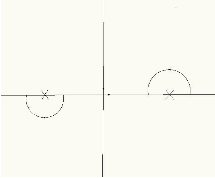
Figure 3.1: The Feynman contour.
