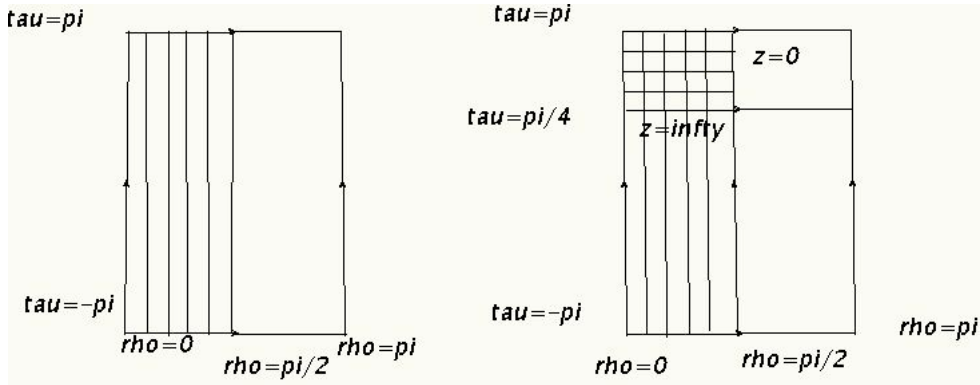
Figure 9.6: Conformal structure of AdS_n . In the figure on the right it is represented the portion of the space covered by Poincaré coordinates.
