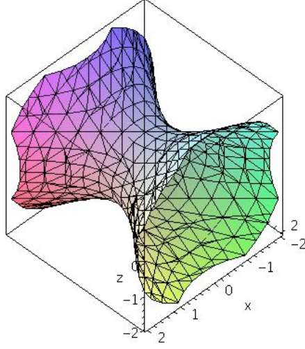
Figure 9.1: A pictorial representation of Anti de Sitter ( X_0^2 + X_1^2 = l^2 + \vec{X}^2 in \mathbb{R}^n ).
