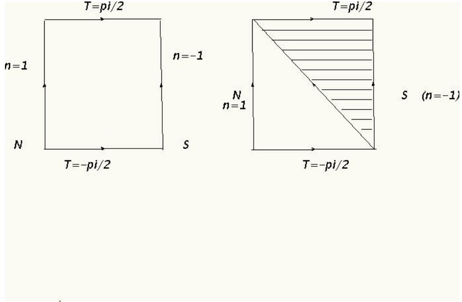
Figure 9.4: Conformal structure of dS_n . In the figure on the right it is represented the portion of the space covered by Poincaré coordinates.
