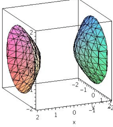
Figure 9.2: A pictorial representation of Euclidean Anti de Sitter (or Euclidean de Sitter) (X_0^2 - X_1^2 = l^2 + \vec{X}^2 \text{ in } \mathbb{R}^n
